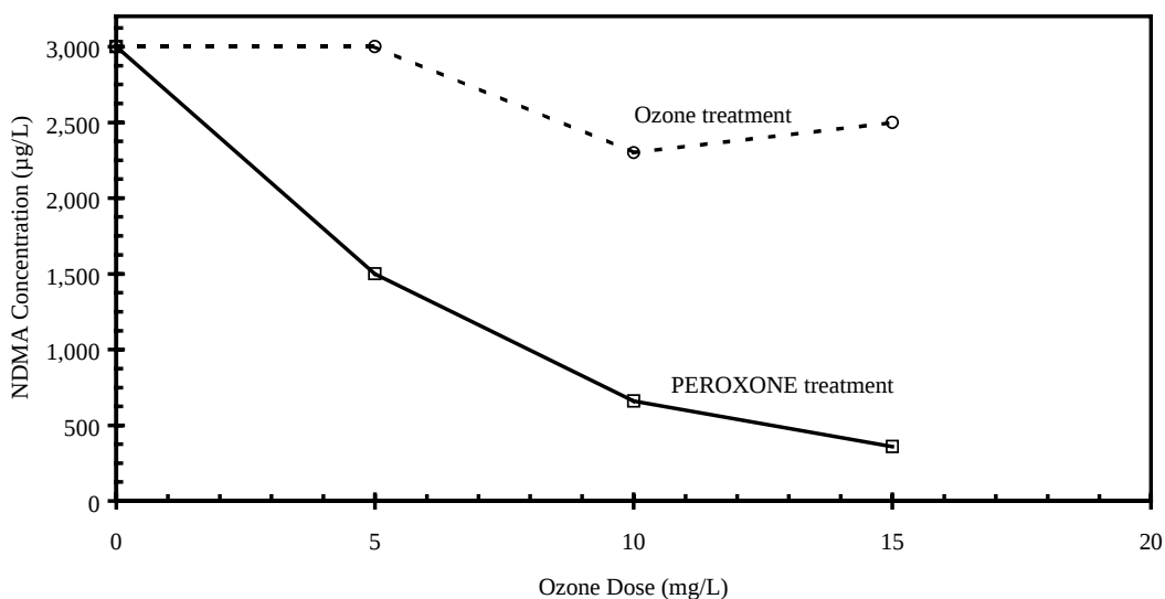
Figure ES3. Effects of Ozone and \text{H}_2\text{O}_2 Dose on NDMA Reduction in Laboratory Water
