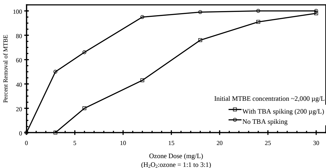
Figure 18. Effect of TBA spiking on MTBE removal (initial MTBE concentration = 2,000 µg/L)
