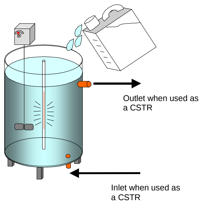
Figure 7. Schematic of the pulsed-UV, continuously stirred tank reactor setup
