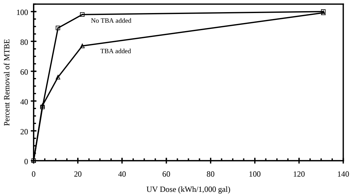
Figure 12. Effect of initial TBA spike on MTBE reduction (25 Hz)
