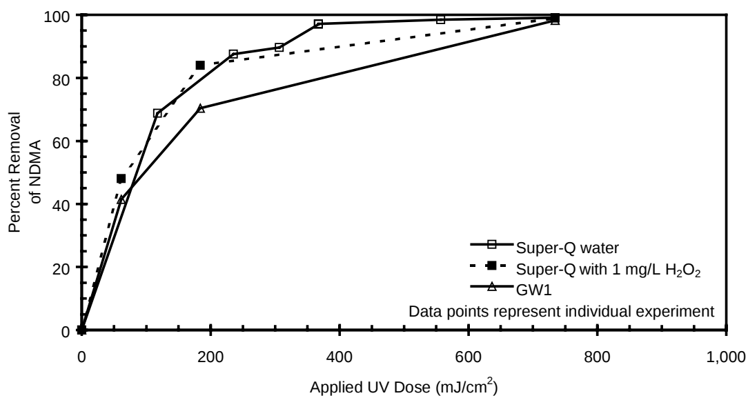
Figure 23. Effect of nitrate on NDMA reduction by UV light in laboratory water
