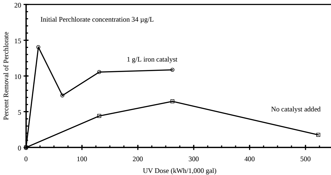
Figure 28. Effect of catalyst addition on perchlorate reduction (laboratory water, pH = 3)
