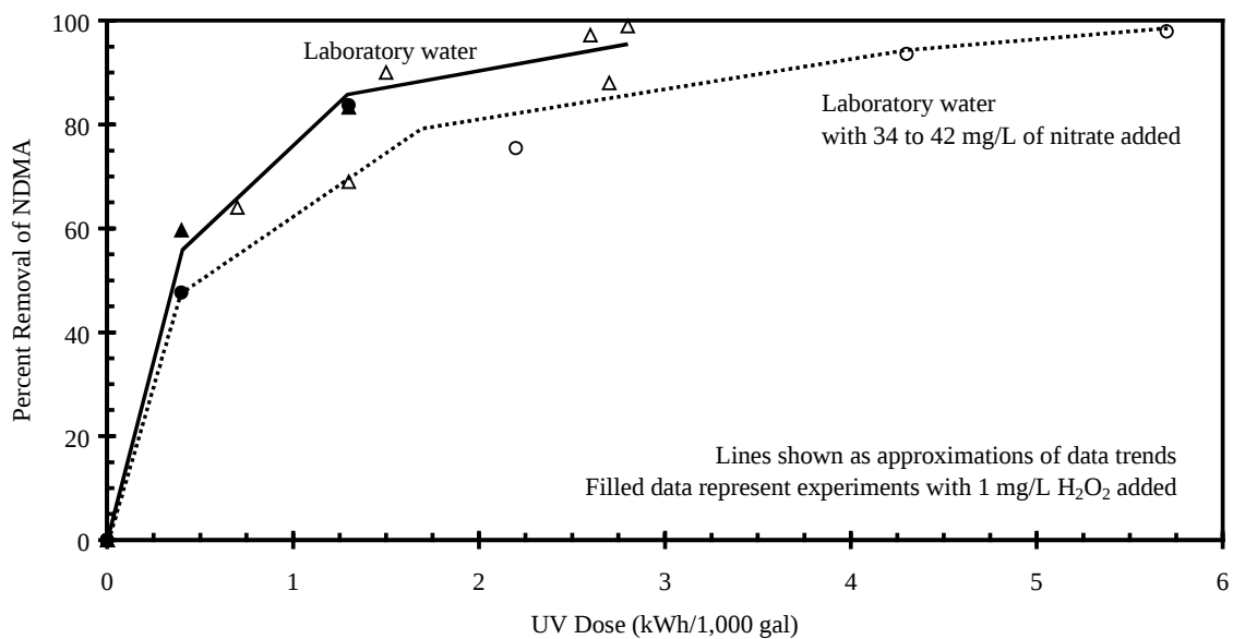
Figure 22. Effect of nitrate on UV treatment of NDMA
