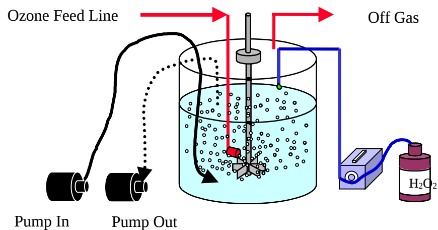
Figure 4. Schematic of the PEROXONE batch reactor (flow through setup)
