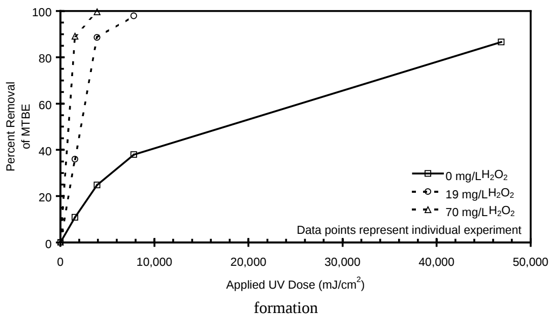
Figure 14. Effect of UV and UV/H 2 O 2 on MTBE
