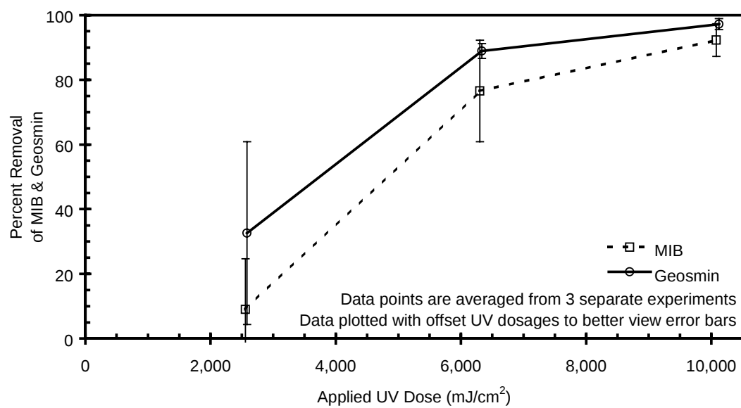
Figure 31. Effect of UV on MIB and geosmin
