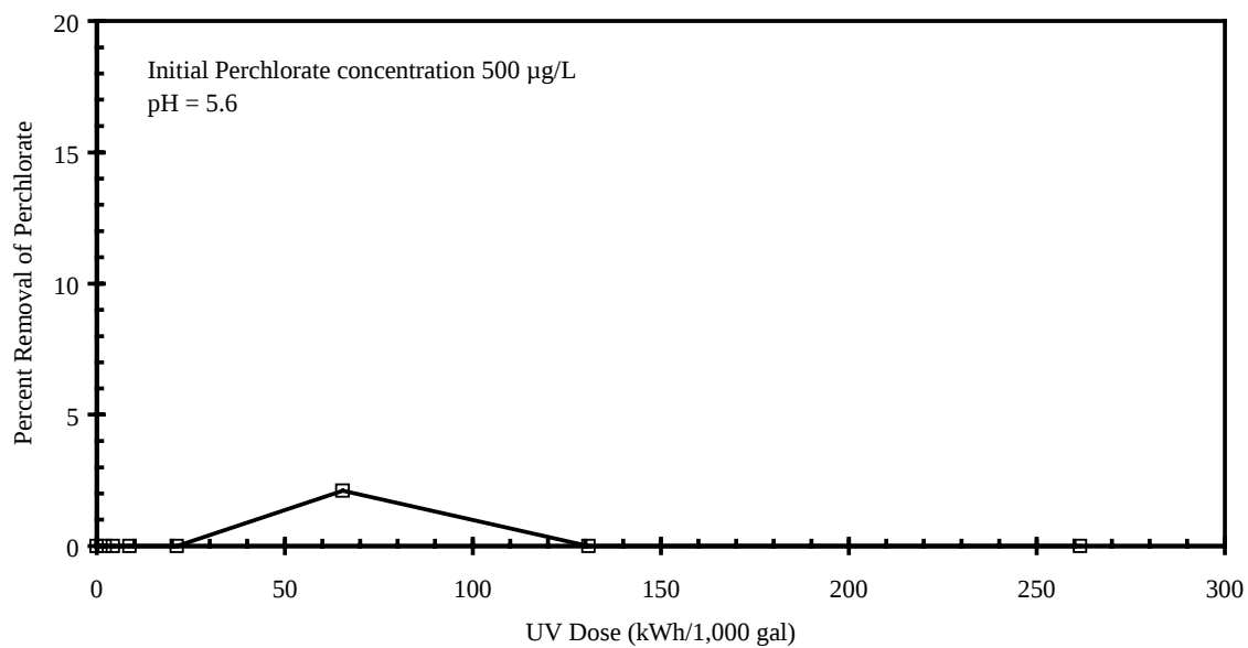
Figure 26. Reduction of perchlorate in laboratory water (25 Hz)
