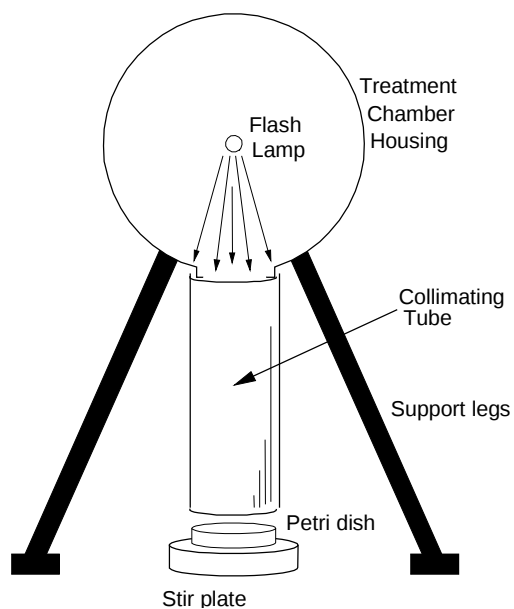
Figure 6. Pulsed-UV, collimated-beam setup for preliminary bromate experiments
