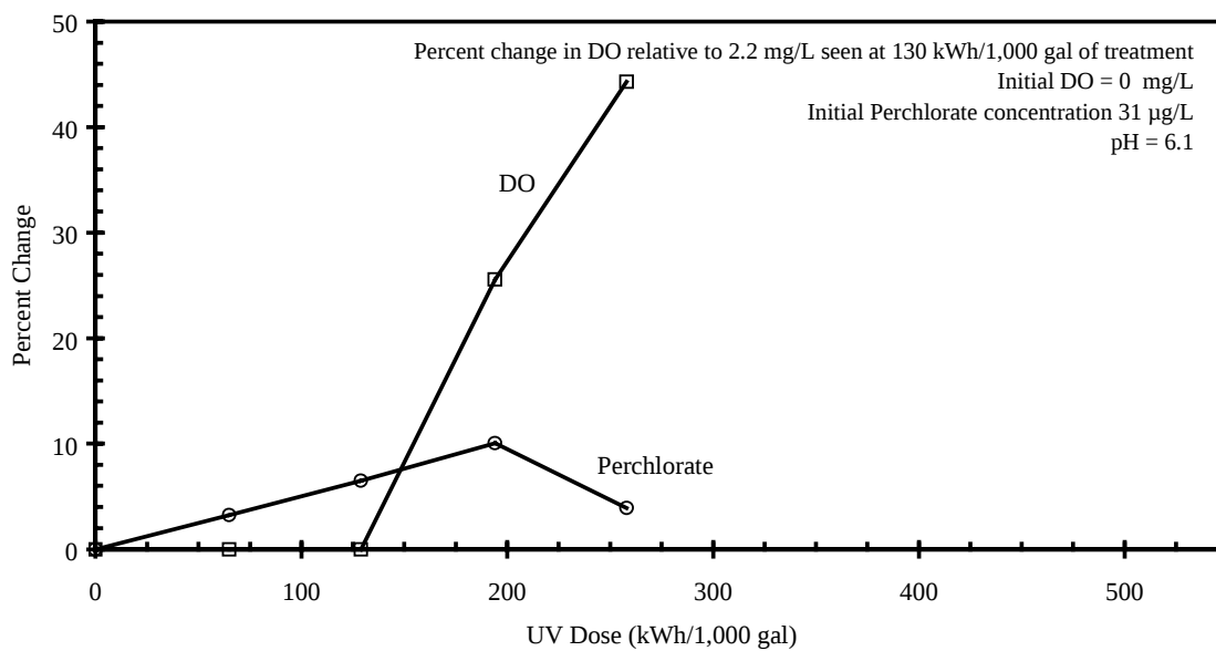
Figure 29. Perchlorate and dissolved oxygen levels during anaerobic treatment
