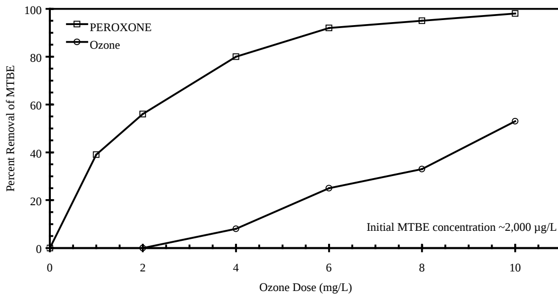
Figure 15. Effect of ozone and PEROXONE on MTBE removal (initial MTBE concentration = 2,000 µg/L)
