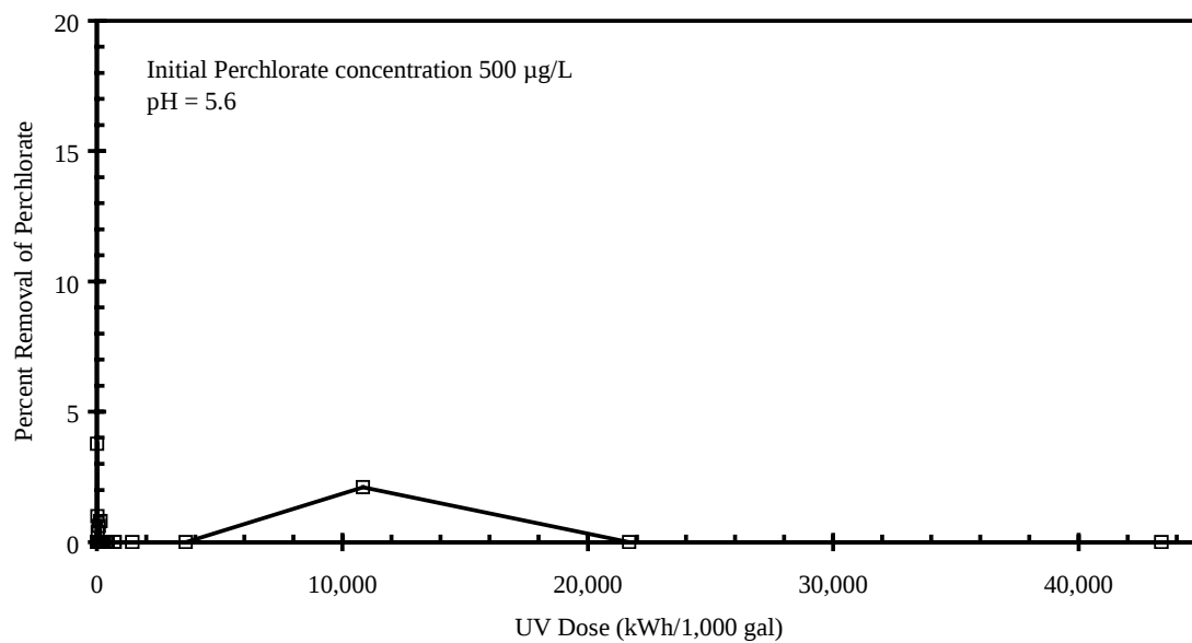
Figure 30. Reduction of perchlorate in laboratory water
