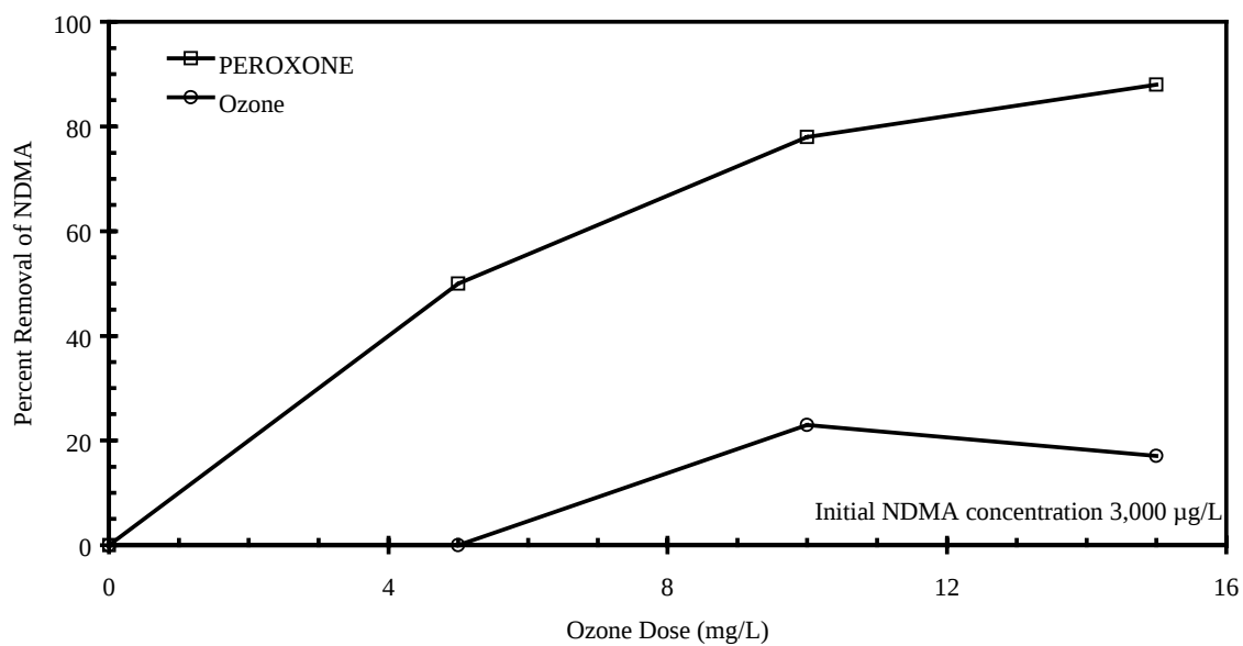
Figure 24. Effect of Ozone and PEROXONE on NDMA reduction
