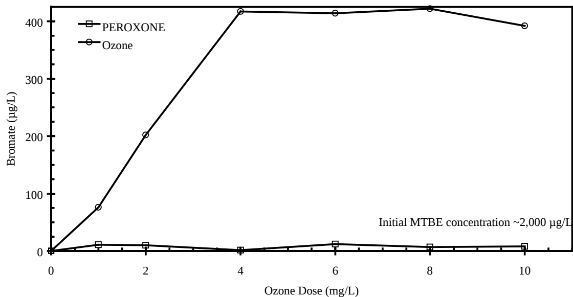
Figure 20. Effect of ozone and PEROXONE on bromate formation (initial MTBE concentration = 2,000 µg/L)
