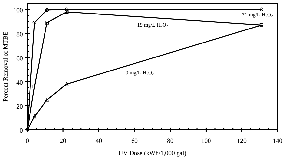
Figure 10. Effect of H 2 O 2 on MTBE percent removal
