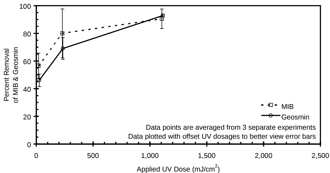
Figure 32. Effect of UV/H 2 O 2 on MIB and geosmin (5.5 mg/L H 2 O 2 )
