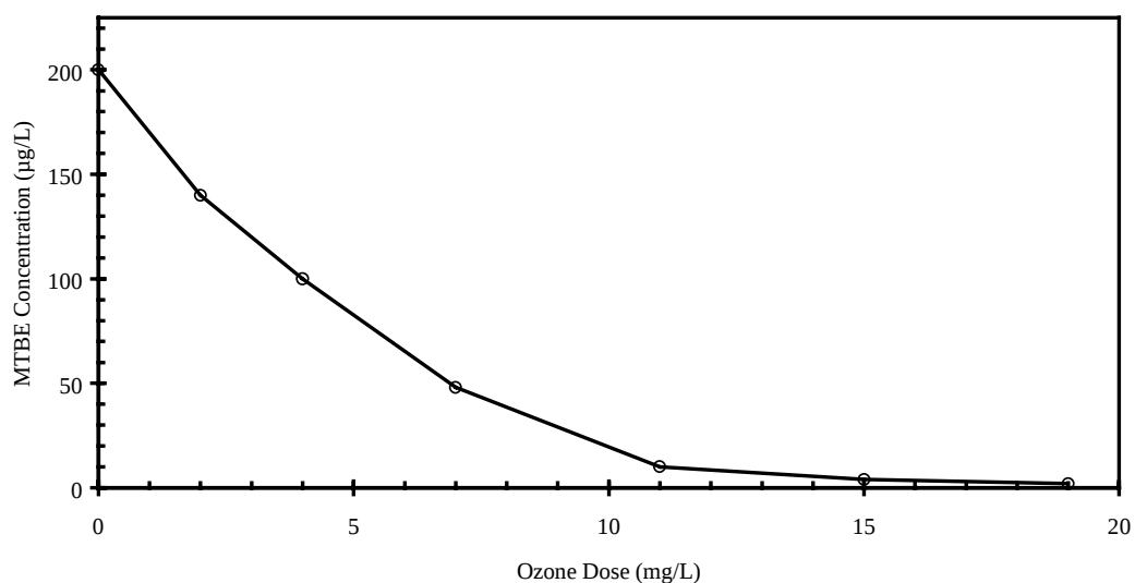
Figure ES2. Ozone Dosage Required to Control MTBE
