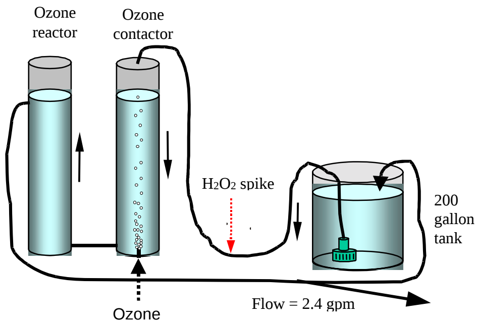
Figure 2. Schematic of ozonation setup for MTBE tests
