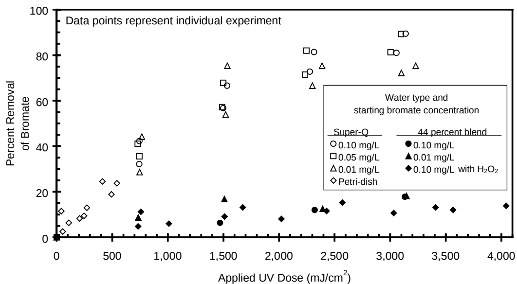
Figure 9. Effect of UV and UV/H 2 O 2 treatment on two waters containing bromate (4.1 mg/L H 2 O 2 dose)
