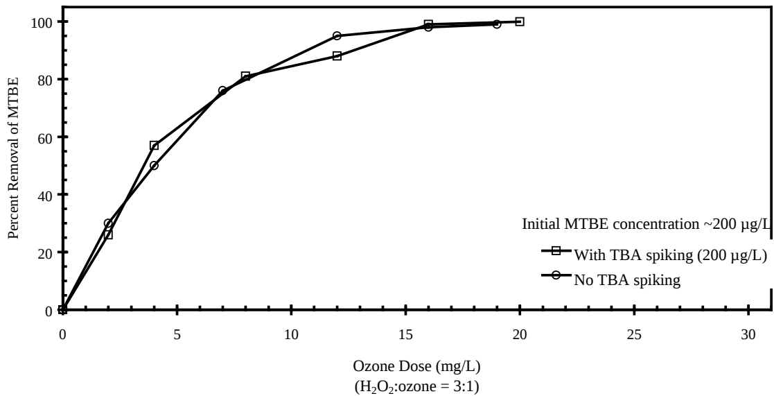
Figure 17. Effect of TBA spiking on MTBE removal (initial MTBE concentration = 200 µg/L)
