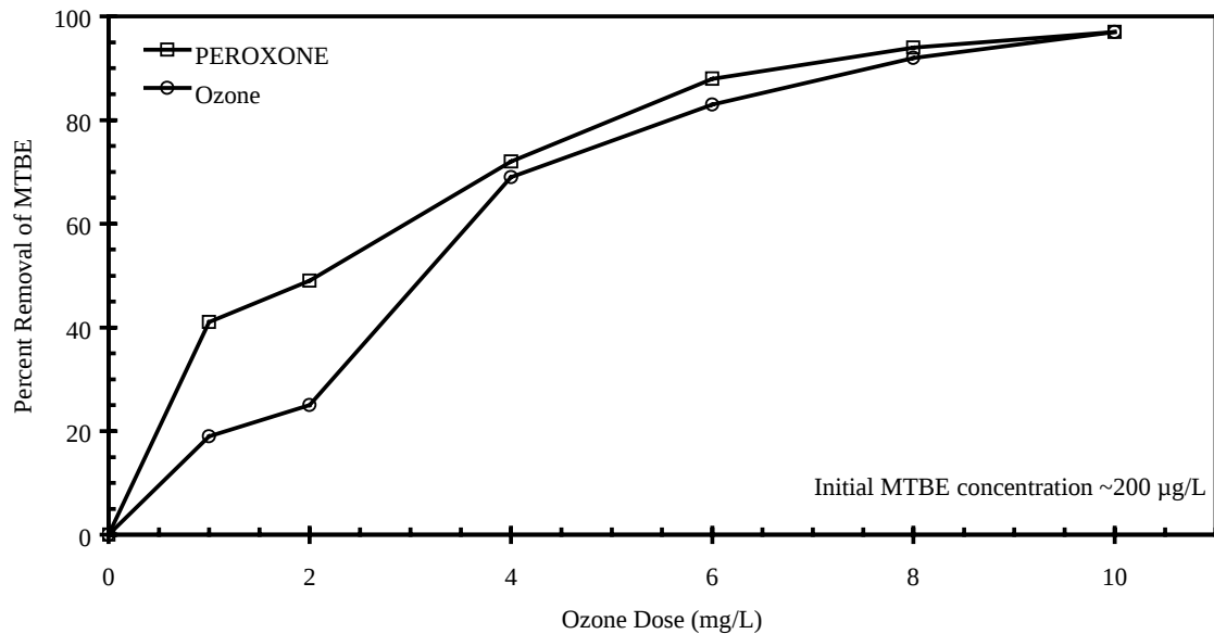
Figure 16. Effect of ozone and PEROXONE on MTBE removal (initial MTBE concentration = 200 µg/L)
