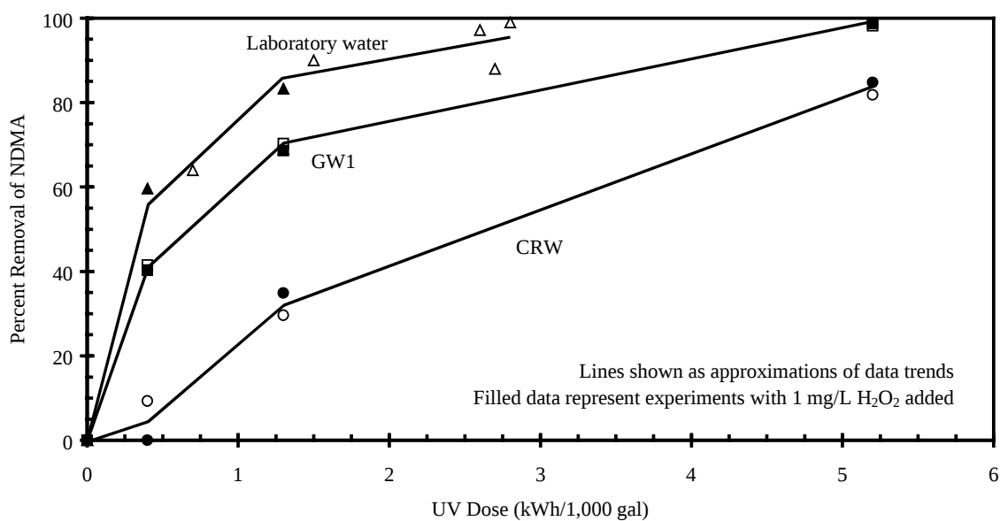
Figure 21. Effect of water type on UV treatment of NDMA
