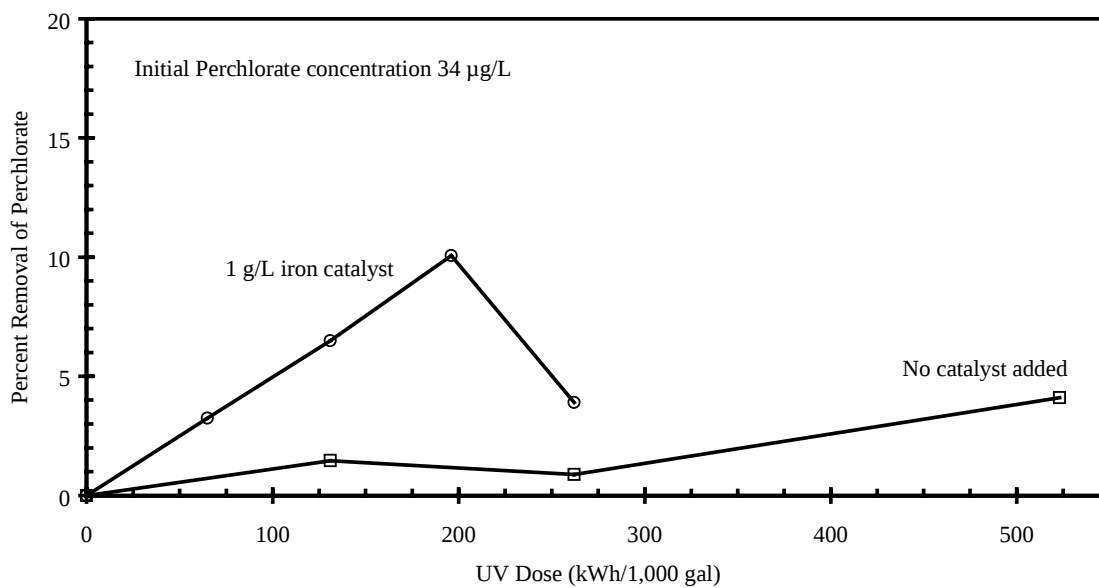
Figure 27. Effect of catalyst addition on perchlorate reduction (laboratory water, ambient pH)
