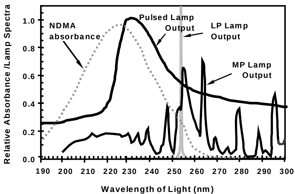
Figure 1. UV lamp output characteristics compared with NDMA light absorbance
