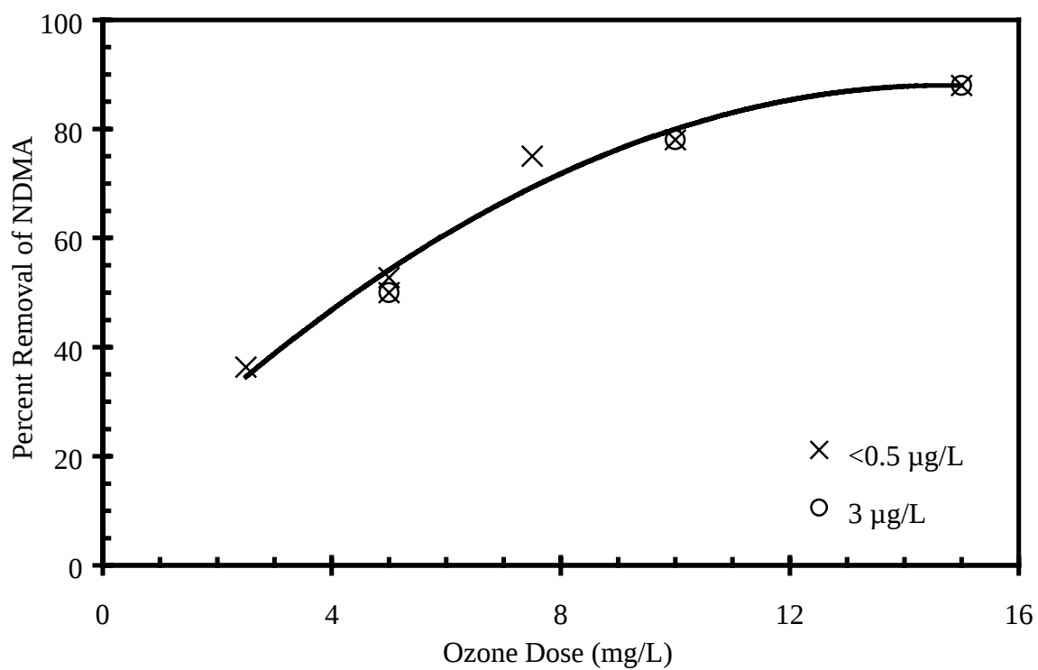
Figure 25. Effect of initial NDMA concentration on treatment by ozone
