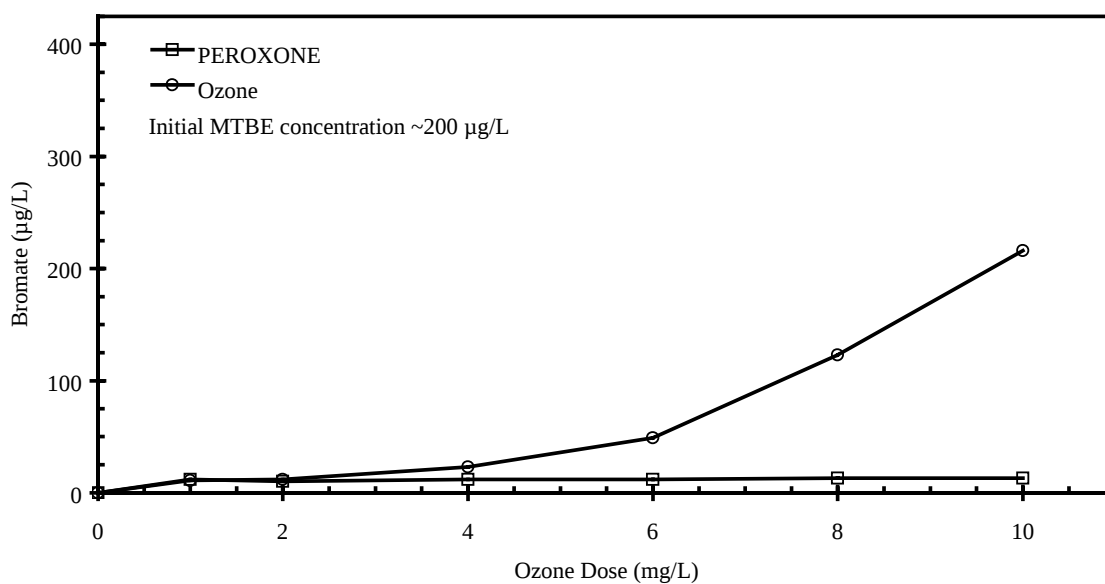
Figure 19. Effect of ozone and PEROXONE on bromate formation (initial MTBE concentration = 200 µg/L)
