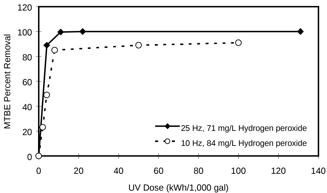
Figure 11. Effect of UV dose (UV frequency) on MTBE percent removal
